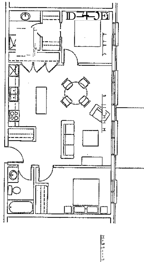
70 s.m. Unit 1:50
